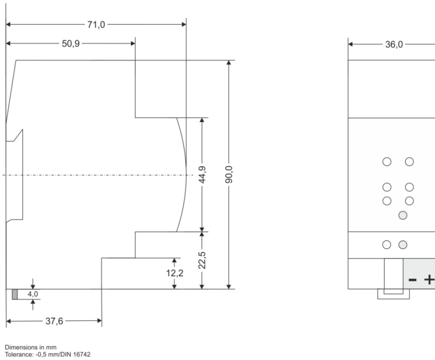
Figure 19: Dimension drawings
