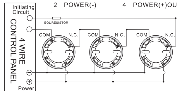
4 wire detectors wiring diagram
