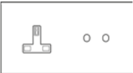
2 Gang frame 85x155,5x4 mm
